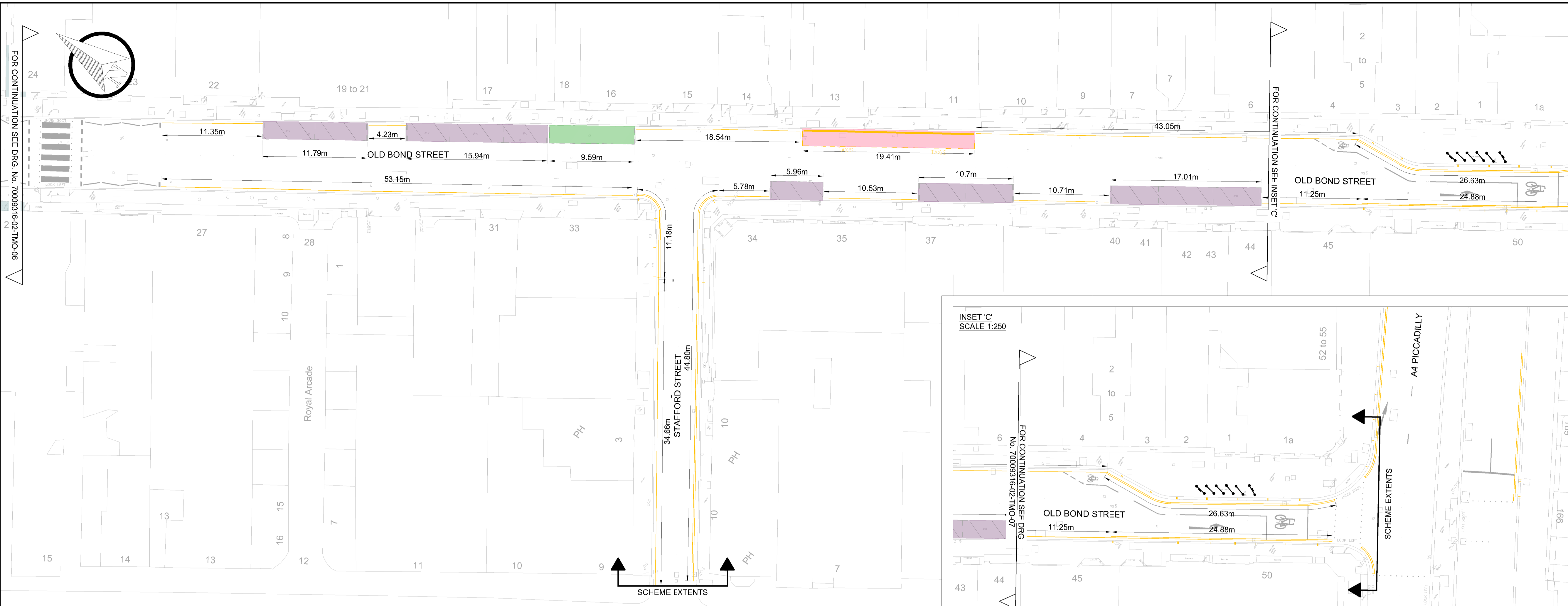
EXISTING TMO LAYOUT SHEET 7
